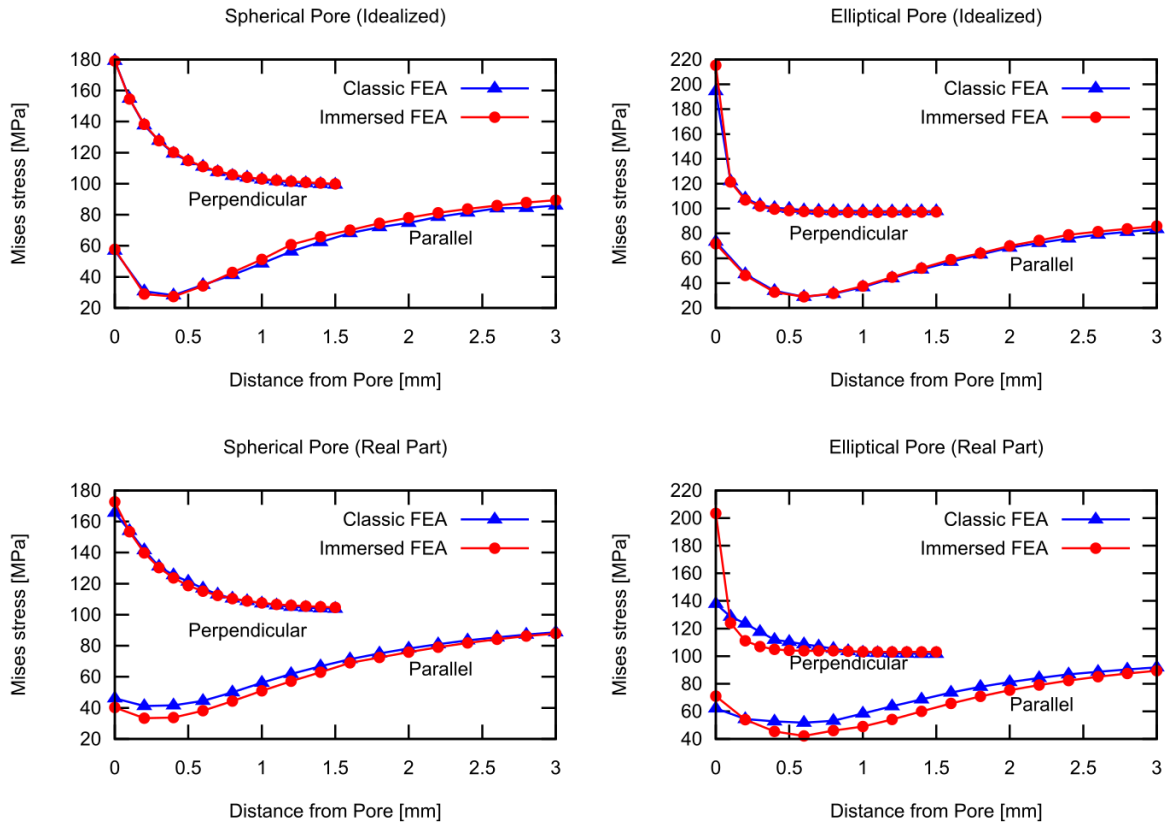
Fig. 4: Top row: For idealized geometries the computed stresses are effectively identical between the classic FEA and the immersed solver. Bottom row: For simulation on CT images of real parts, the immersed method takes more geometric details in to account and thus yields more accurate results.
