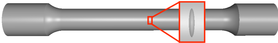
Fig. 2: CAD model of the test specimen. A pore is inserted at the centre of symmetry (elliptical version shown here).
