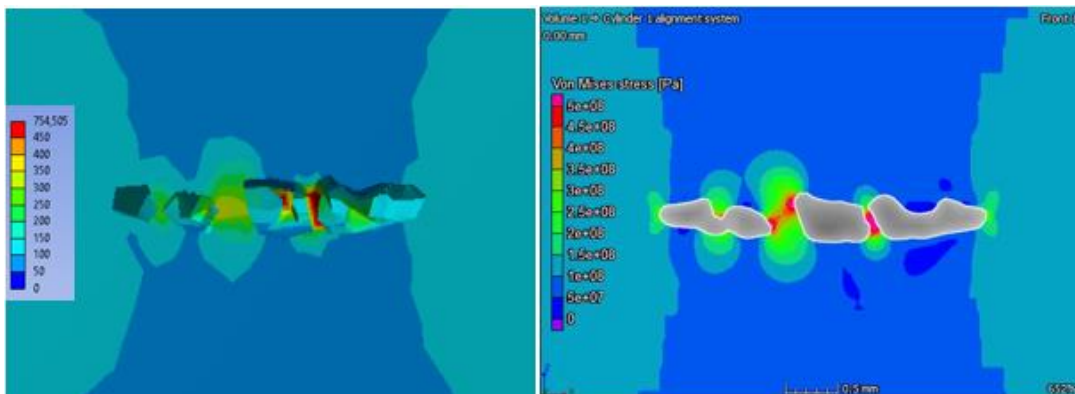
Fig. 5: Mises stress on a 2D section through the elliptical pore. Left: Classical FEA, Right: Immersed method.
