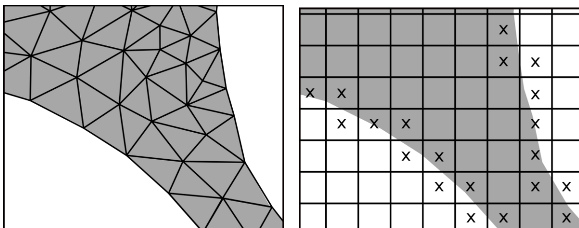
Fig. 1. Left: Classical FEA: The shaded area is a detail of a complex simulated object. The object is represented by a geometry-conforming mesh (black lines). Right: Immersed method. The simulation domain is extended beyond the object borders and discretized by a trivial quadrilateral mesh (black lines). The mesh cells cutting through the object boundary (marked with crosses) are treated in a special way to regard the exact object surface (no "Lego"-brick model!)
